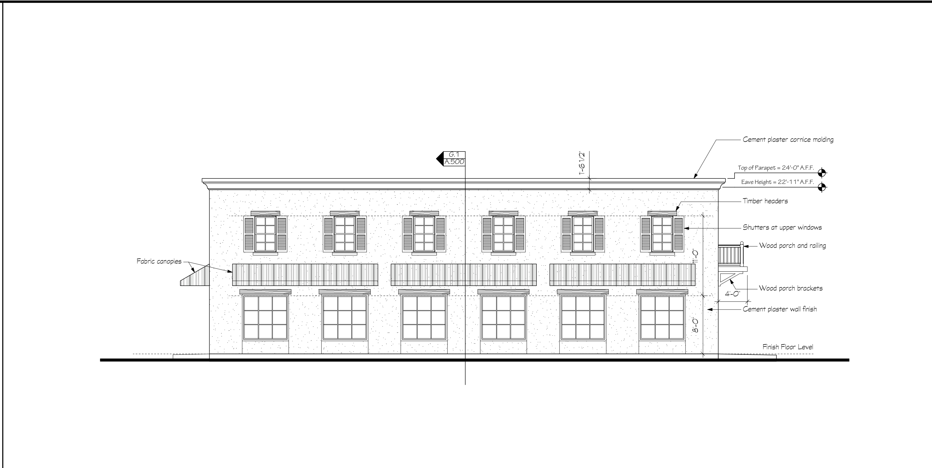
J.9 Building Elevation (South-Albertson's Parkway Side) Scale: 1/8" = 1'-0"
